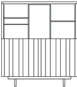
Cabinet Art. 80120 120 x 52 x H 133 cm
